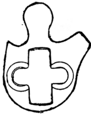
XL12-304 “Classic” Keyway non-handed ( countersunk ) ( both sides )
